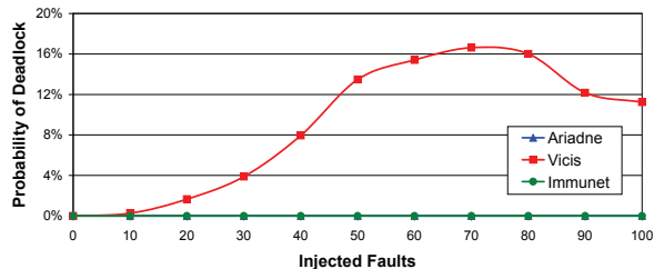
Fig. 10: Probability of deadlock over different fault configurations. Ariadne, Immunet are deadlock free (lines overlap at the 0% value), while Viciis is not.
