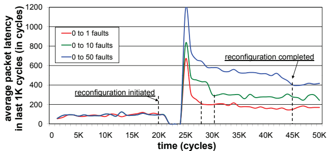
Fig. 11: Reconfiguration dynamics. Average packet latency over time, assuming uniform random traffic, 0.1 injection rate.
